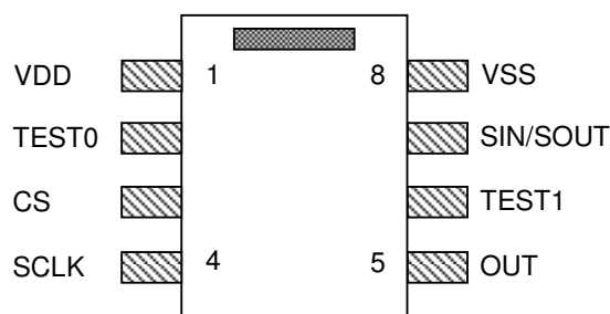
Figure 2. Pin Configuration
